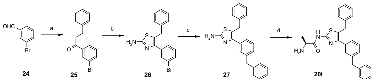
Scheme 2. Reagents and conditions: (a) (i) phenethylmagnesium chloride, THF; (ii) (COCl) 2 , DMSO, TEA, DCM, –78 °C; (b) (i) Br 2 , AcOH, CHCl 3 , rt; (ii) thiourea, EtOH, reflux; (c) benzylzinc bromide, Cl 2 Pd(dppf), THF, reflux; (d) (i) BOC-Ala-OH, EDC, HOAt, DCM; (ii) 50% TFA, 5% TES-H, DCM.
