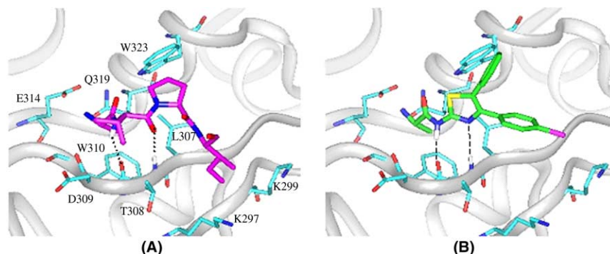
Figure 1. (A) A ribbon depiction of the AVPI terminus of the SMAC peptide bound to the BIR3 domain of XIAP (PDB ID: 1G3F). The peptide is colored magenta. Residues that make important contacts are rendered. Earlier SAR indicates that the N-terminal amino, the Ala-Val peptide bond, the carbonyl of the Val-Pro peptide bind and the hydrophobic interactions of the Ile and Pro are important for tight binding. (B) Model of 20g docked into the Bir3/SMAC peptide structure. Fifteen NOEs between 20g and the protein were used to define its orientation.
