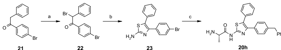
Scheme 1. Reagents and conditions: (a) Br 2 , AcOH, CHCl 3 , rt; (b) thiourea, EtOH, reflux; (c) (i) benzylzinc bromide, Cl 2 Pd(dppf), THF, reflux; (ii) Boc-Ala-OH, EDC, HOAt, DCM; (iii) 50% TFA, 5% TES-H, DCM.
