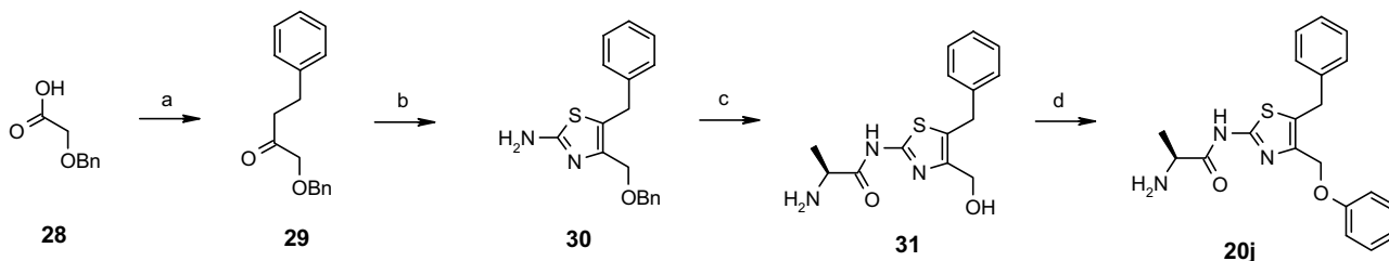
Scheme 3. Reagents and conditions: (a) (i) (COCl) 2 , DMSO, TEA, DCM, –78 °C; (ii) phenethylzinc bromide, Pd(PPh 3 ) 4 , THF, reflux; (b) (i) TESOTf, TEA, DCM, –10 °C to rt; NBS, THF; (ii) thiourea, EtOH, reflux; (c) (i) Boc-Ala-OH, EDC, HOAt, DCM; (ii) BCl 3 -DMS, DCM, –78 °C; (d) (i) (BOC) 2 O, NaHCO 3 , dioxane, rt; (ii) phenol, diisopropyl azodicarboxylate, PPh 3 , THF, 0–55 °C; (iii) 50% TFA, 5% TES-H, DCM.
